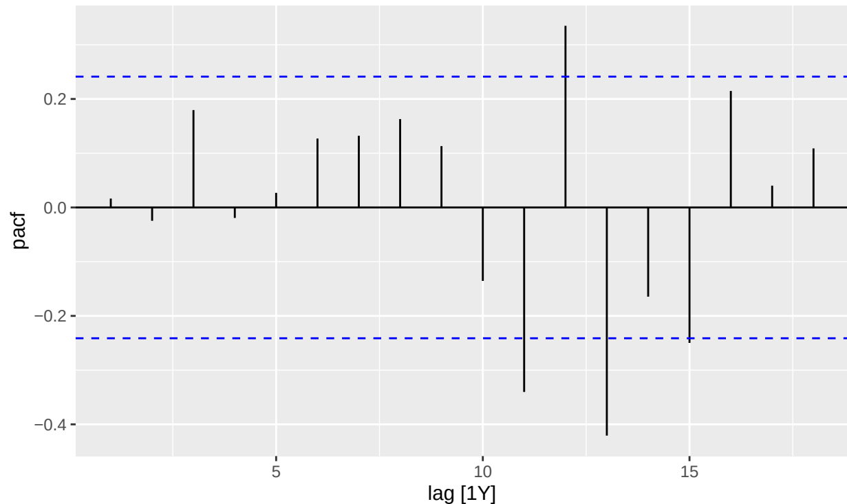
Figure 9. Partial Autocorrelation Function of the stationary Total Fertility Rate data in Singapore from 1960–2024.
