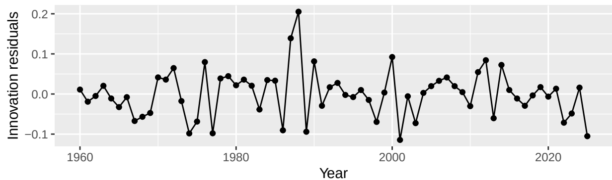
1960–2024 TLB ARIMA (0,1,0) Plots
