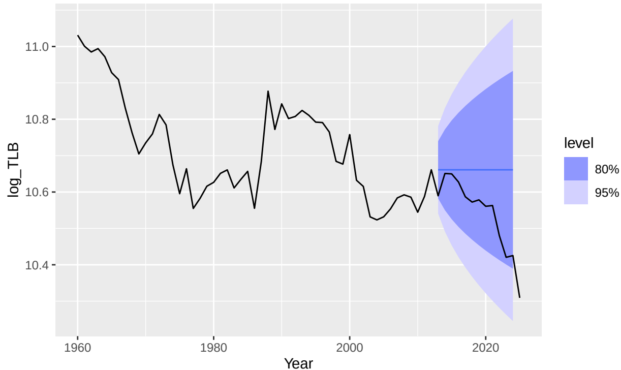
Figure 14. Plot shows that the ARIMA model predicts a straight line for the log of the TLB in Singapore from 2013–2024.
