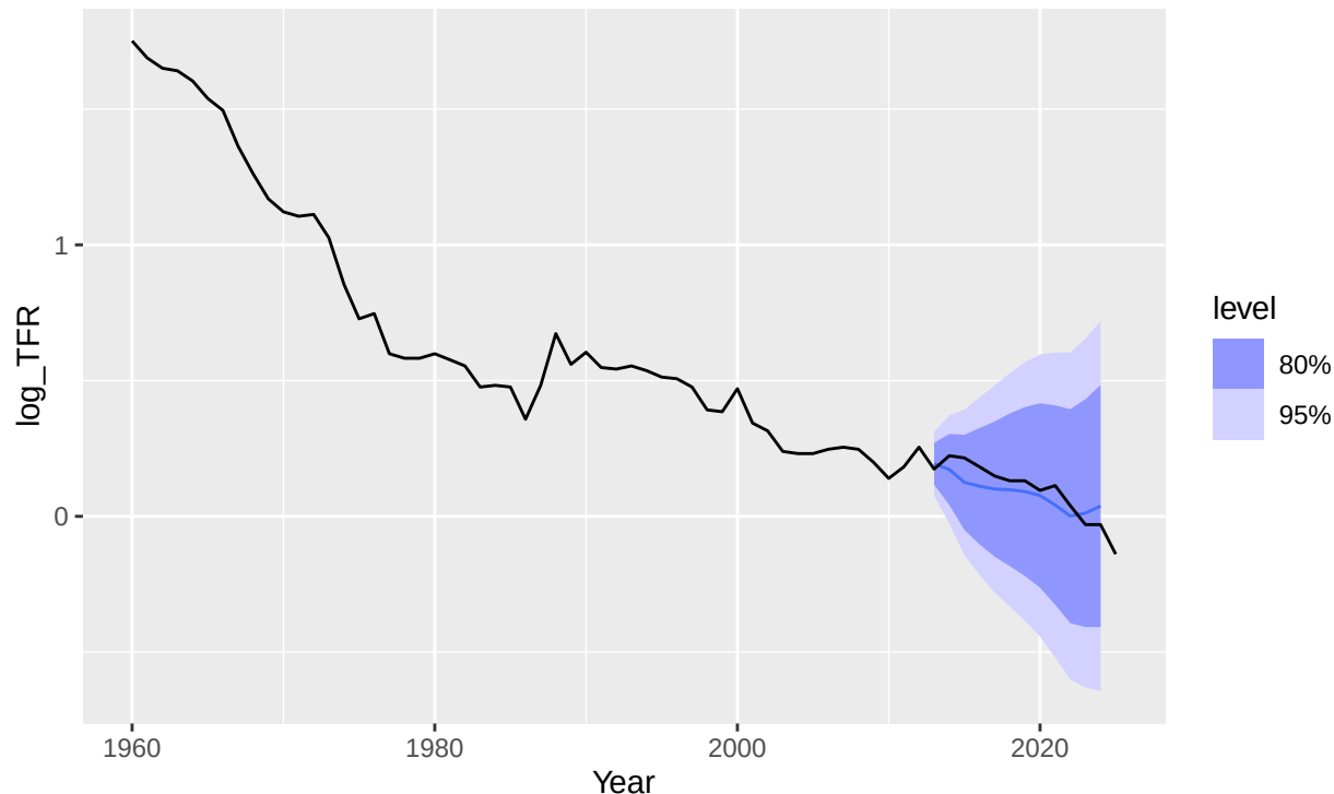
Figure 15. Plot shows that the SARIMA predictive model shows on par fertility rates in singapore from 2013–2024 with the known data.
