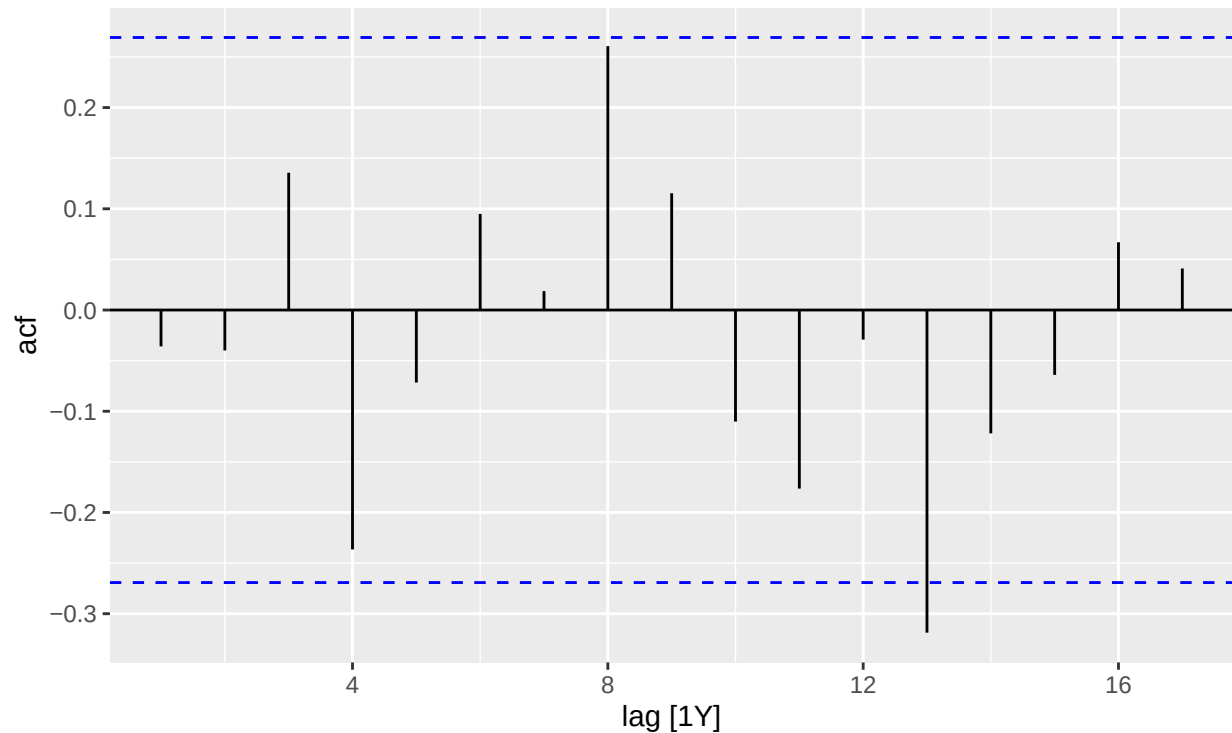
Figure 17. ACF Plot of the SARIMA model shows that there is a spike only at lag 13.
