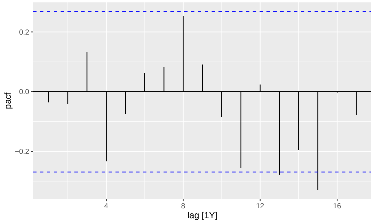
Figure 18. PACF Plot of the SARIMA model shows that there is a spike at lag 15 and potentially at lag 13.
