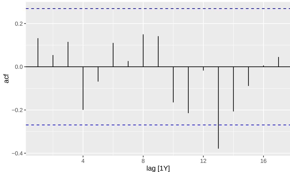
Figure 19. ACF Plot of the predictive SARIMA shows that there is a spike only at lag 13.
