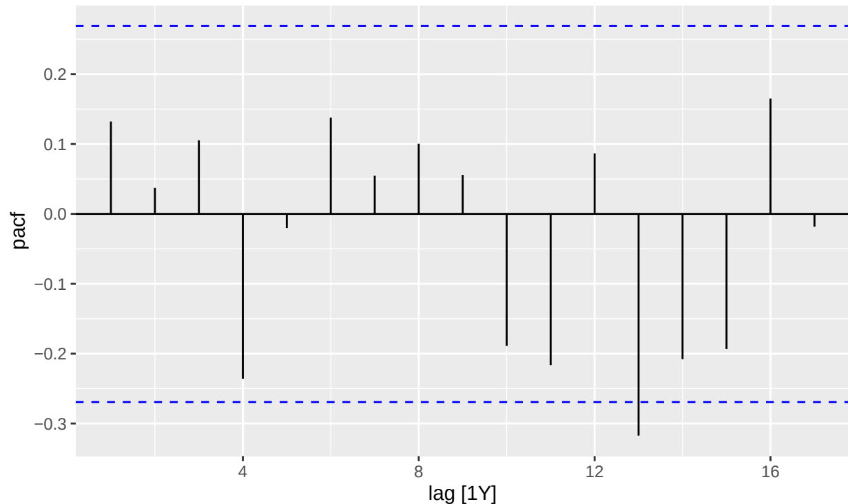
Figure 20. PACF Plot of the predictive SARIMA shows that there is a spike only at lag 13.
