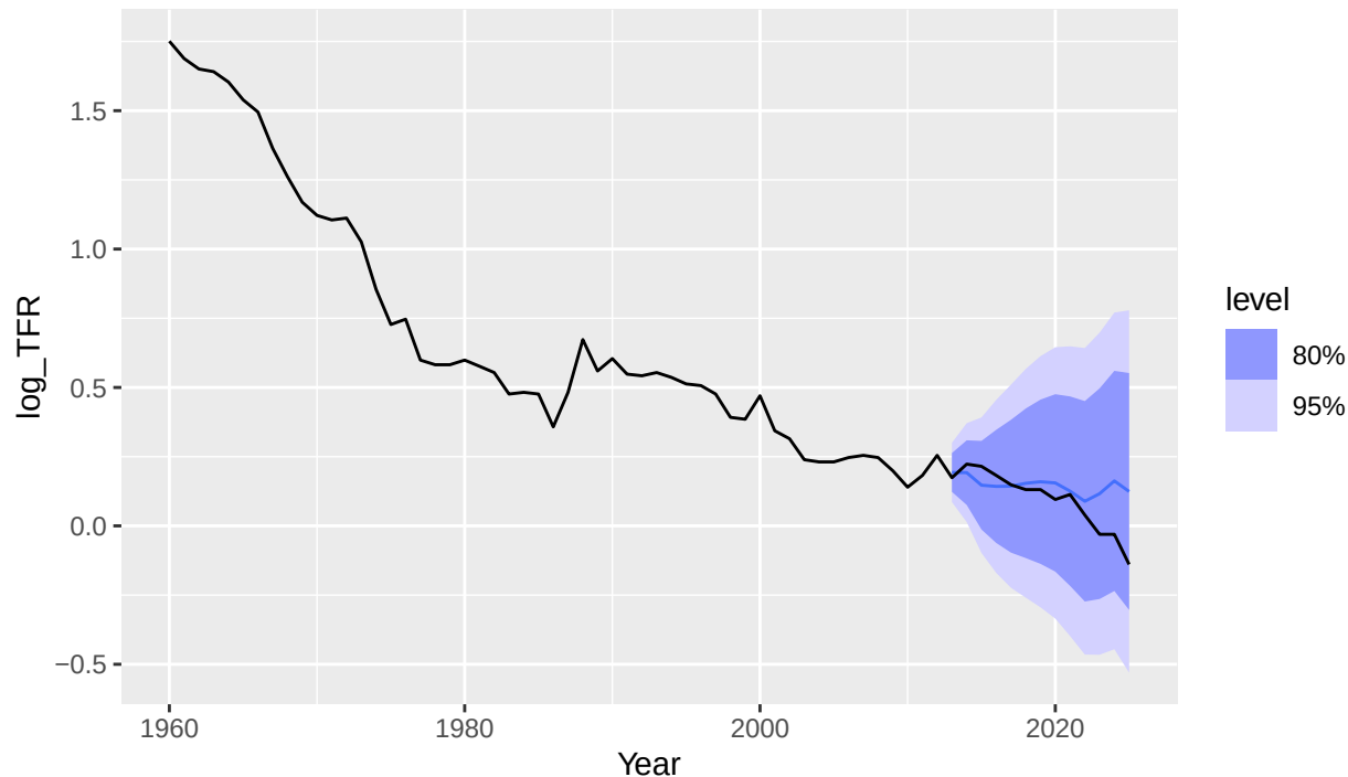
Figure 21. Plot of the predictive SARIMA shows that the SARIMA model that takes the government's family planning policies into account, follows the known TFR data fairly well.
