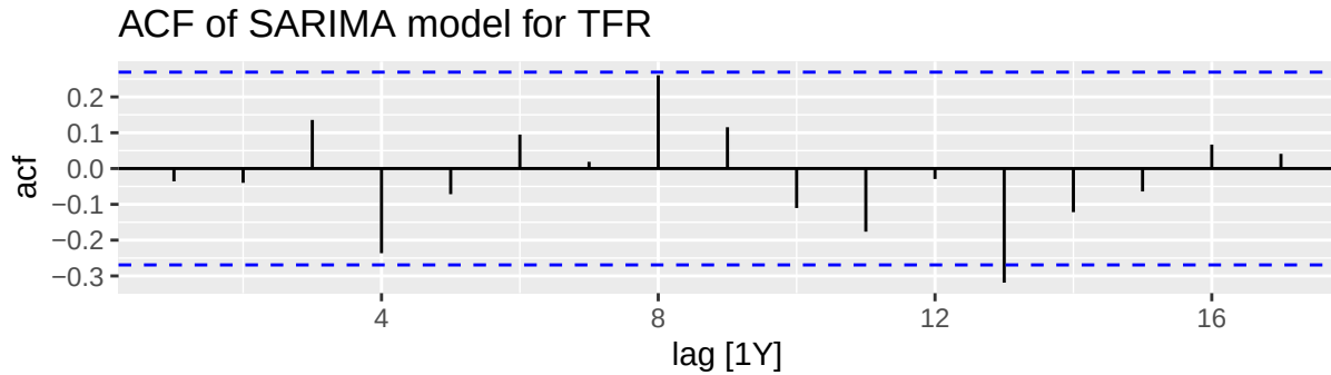
Fig. 17. ACF Plot of the SARIMA model shows that there is a spike only at lag 13.
