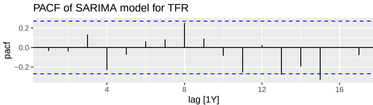
Fig. 18. PACF Plot of the SARIMA model shows that there is a spike at lag 15 and potentially at lag 13.
