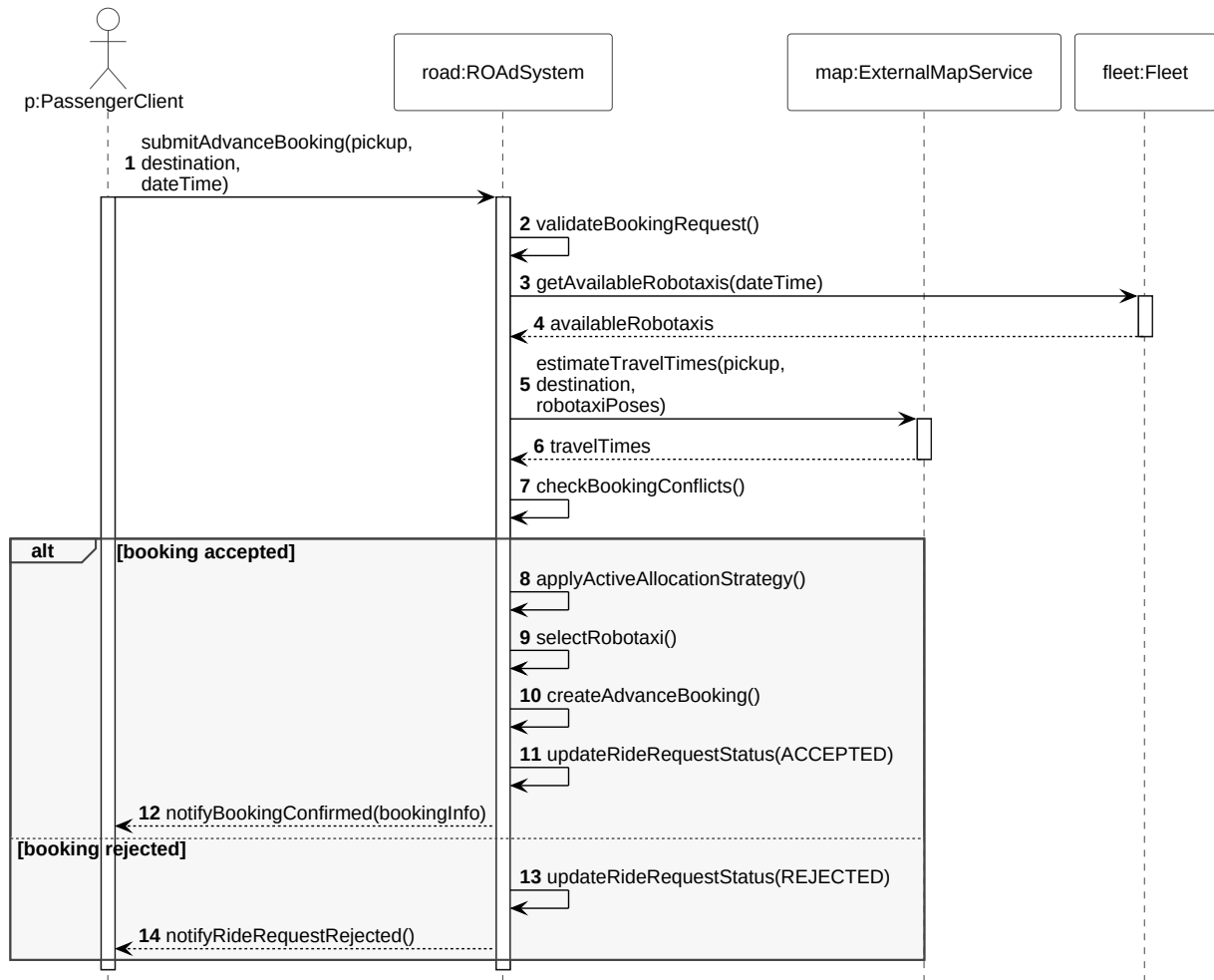
Figure 3.2: Requirements-level sequence diagram for advance ride booking
