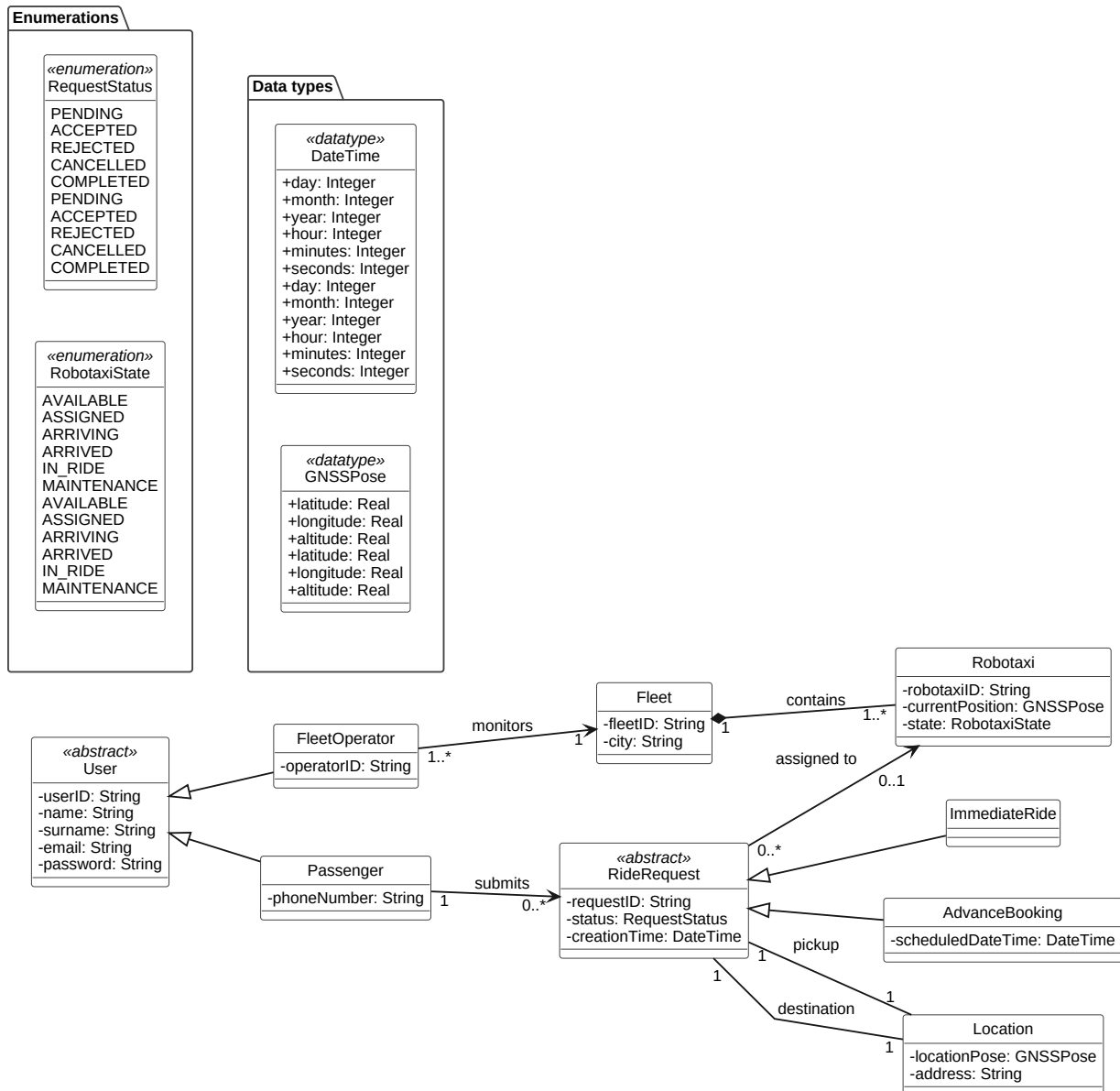
Figure 2.1: Core ROAd domain entities
