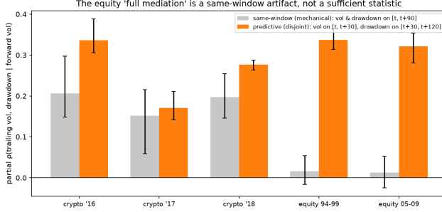
Figure 2: Mediation: partial \rho (trailing vol, drawdown | forward vol). The same-window (mechanical) design gives \approx 0 on equity, falsely suggesting full mediation. The predictive (disjoint-window) design gives 0.32–0.34, so forward volatility does not fully screen off trailing volatility.
