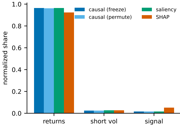
Figure 4: Real agent: normalized per-feature group shares by method. All four tracks agree the recent-returns block dominates the de-risking decision; SHAP places slightly more mass on the salient signal than the causal tracks do, the same bias seen synthetically.
