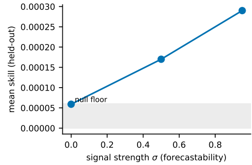
Figure 2: Synthetic skill vs. signal strength (gate). Mean held-out skill rises monotonically with forecastability and collapses toward the noisy null floor (shaded band) at \sigma = 0 , exactly the behaviour a valid skill measure must show.
