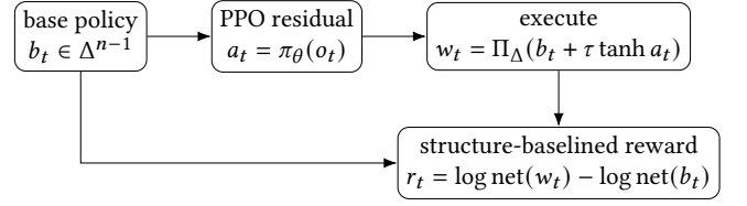
Figure 1: Structure-baselined residual architecture. The base is nested inside the policy ( a_t = 0 \Rightarrow w_t = b_t ), and the reward credits only the agent’s net-log-return increment over the base on the same market path.
