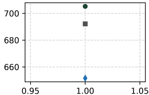
(c) SWEBench
