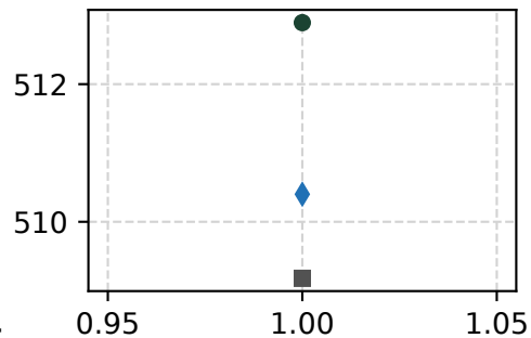
(a) LMSys
