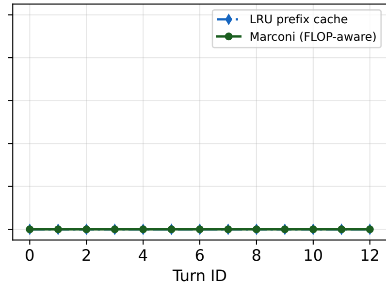
SWEBench
