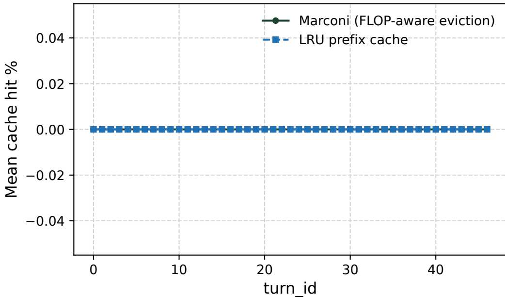
LMSys sps=1.0 (lmsys_sps=1_nums=100.jsonl)
