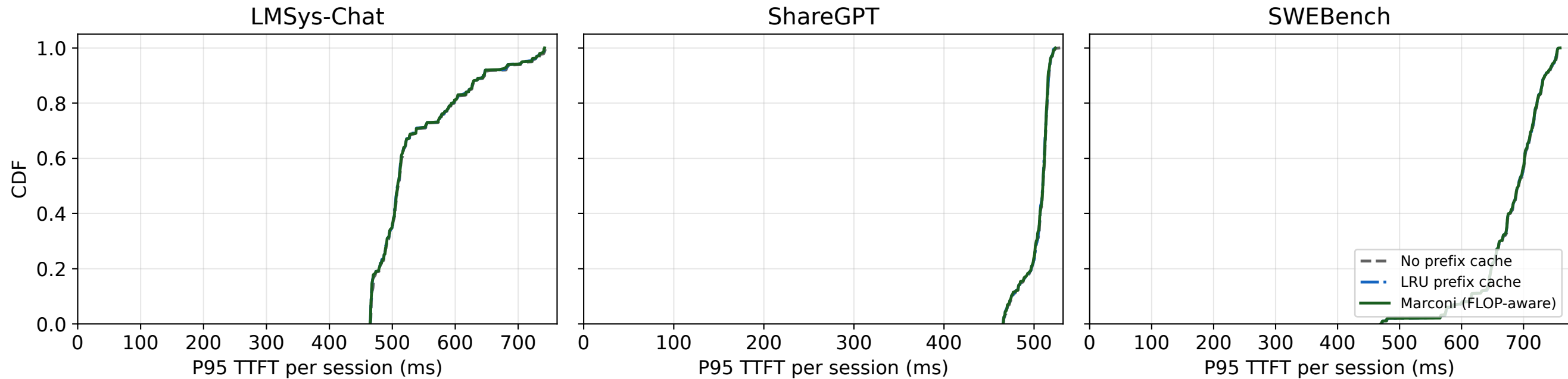
Empirical CDF of TTFT — per session P95 (Fig 10b style)
