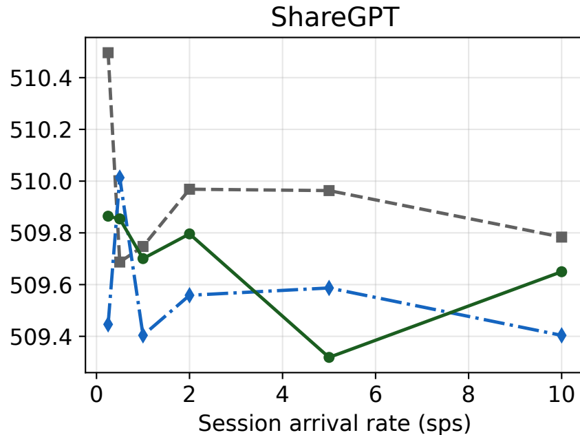
Median of per-session P95 TTFT vs Arrival Rate (Fig 13 style)
