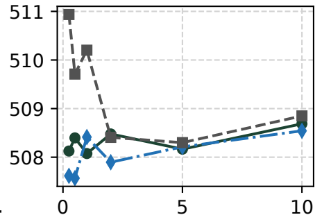
(a) LMSys
