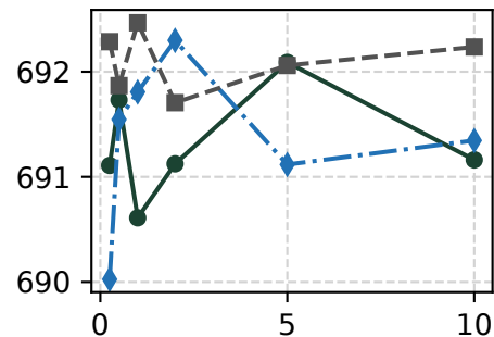
(c) SWEBench
