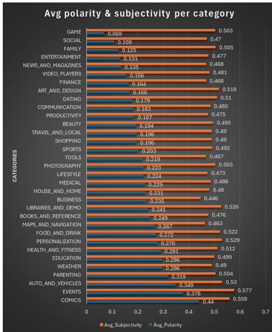
Chart 2: Avg Polarity & Subjectivity per Category (Bar Chart)
