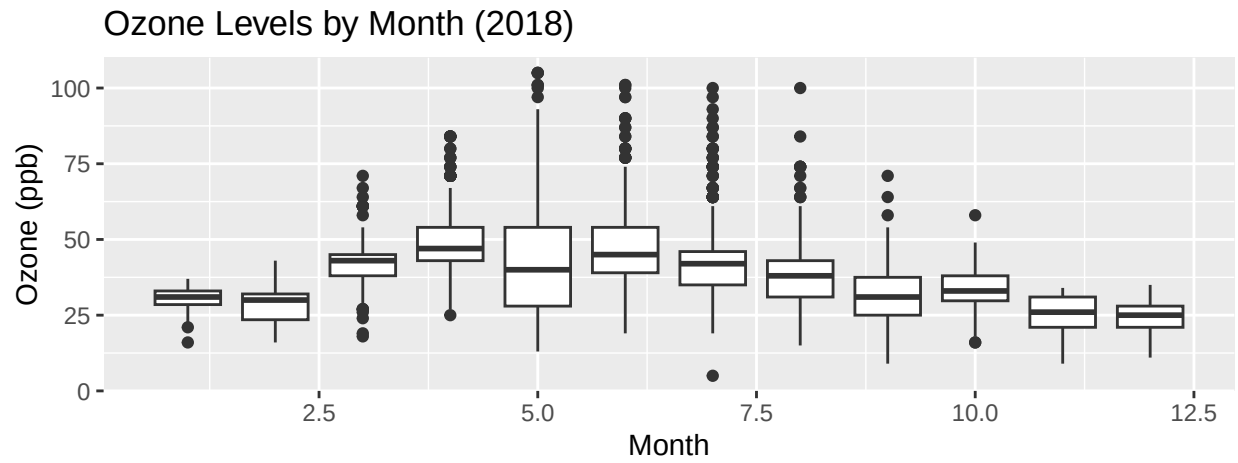
Figure 1: Ozone Levels by Month (2018)
