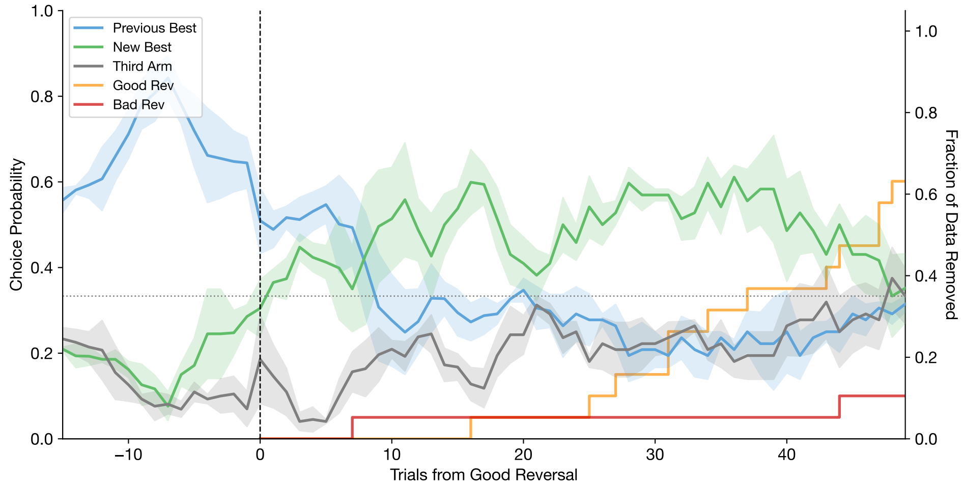
Good Reversal-Aligned Choices (mean \pm se across subjects | n=3 subjects, n=19 reversals)
