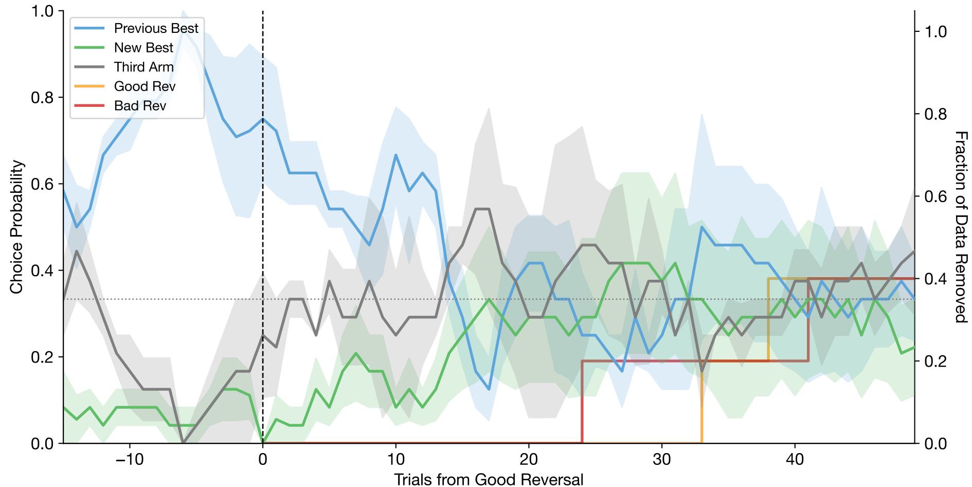
Good Reversal-Aligned Choices (mean \pm se across subjects | n=3 subjects, n=5 reversals)
