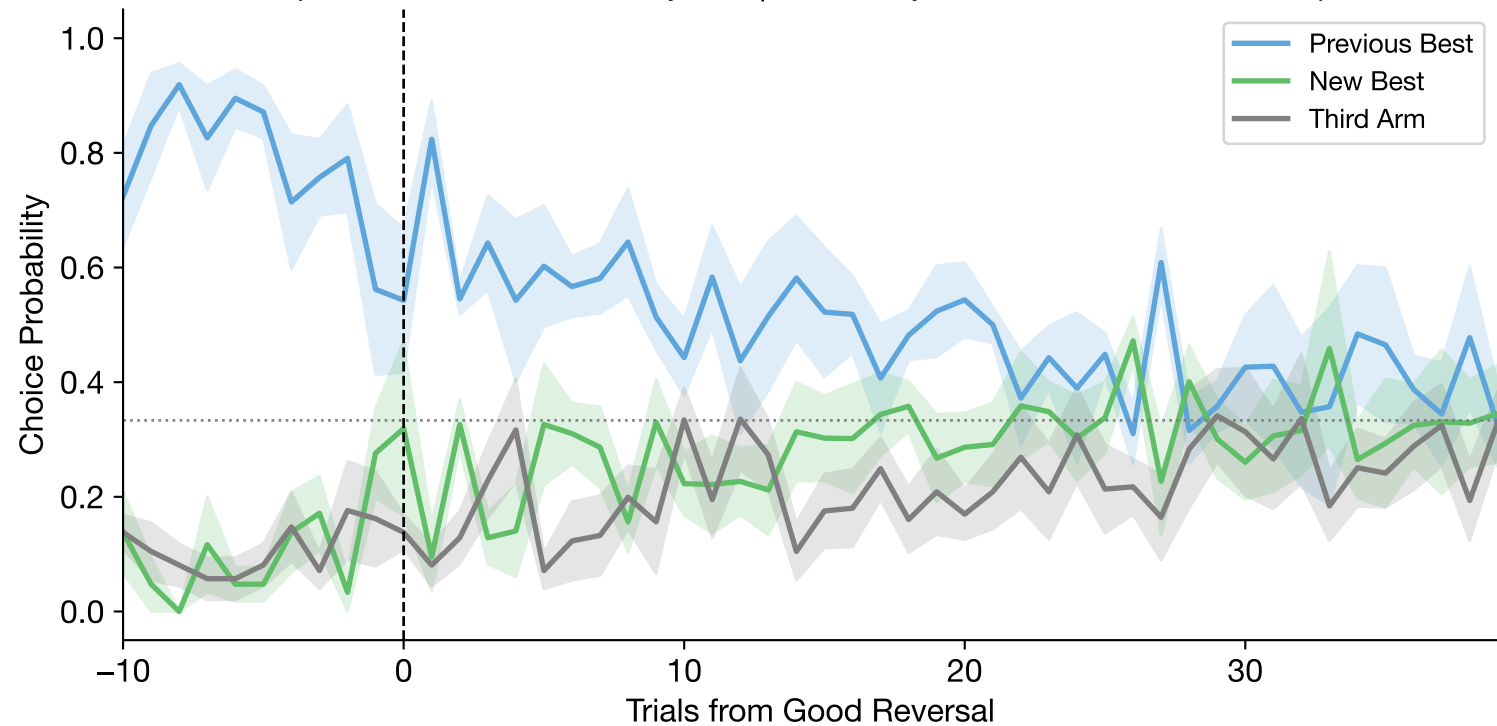
Good Reversal-Aligned Choices (mean \pm se across subjects | n=6 subjects and n=33 reversals)
