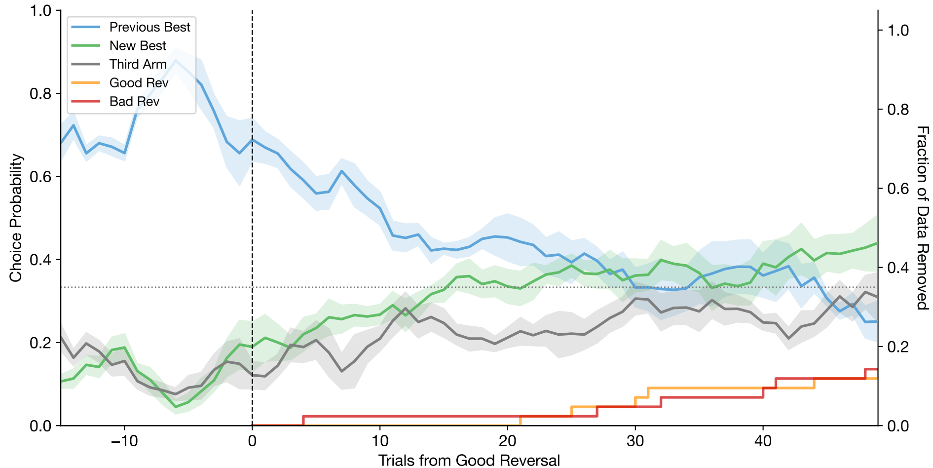
Good Reversal-Aligned Choices (mean \pm se across subjects | n=6 subjects, n=42 reversals)
