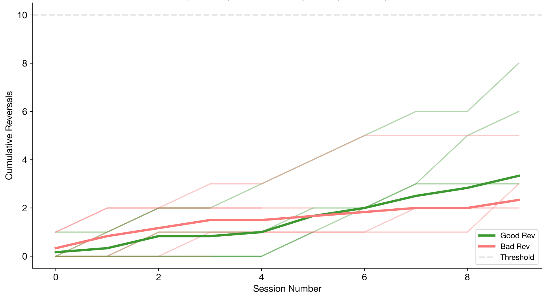
Cumulative Good and Bad Reversals Over Time (n=6 subjects; sessions per subject=4–10)
