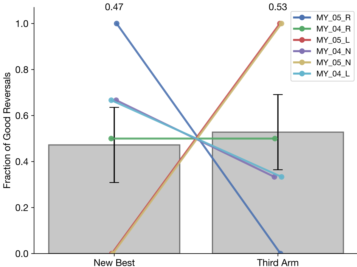
First Choice After Leaving Previous Best (mean \pm se across subjects | n=6 subjects and n=14 reversals)
