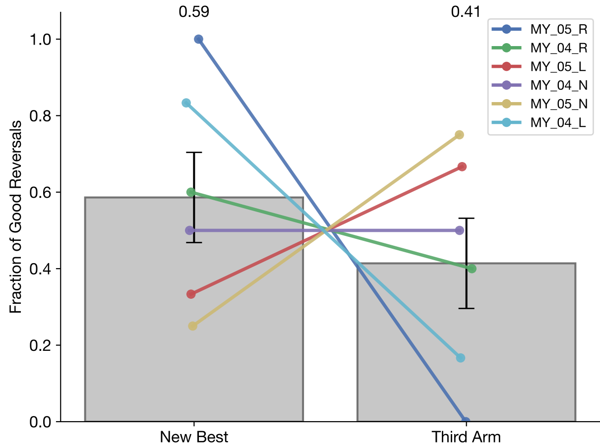
First Choice After Leaving Previous Best (mean \pm se across subjects | n=6 subjects and n=29 reversals)
