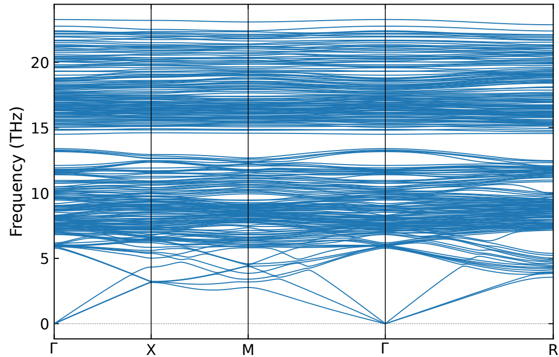
Phonon bands — nodef
