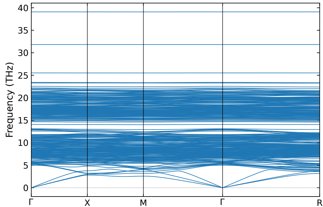
Phonon bands — 2G
