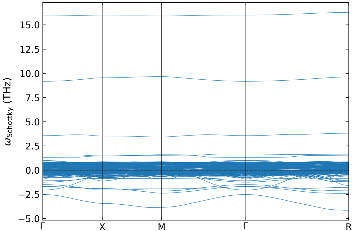
Schottky phonon bands: \omega_{2G} + \omega_{cVac} - 1.96875 \omega_{nodef}
