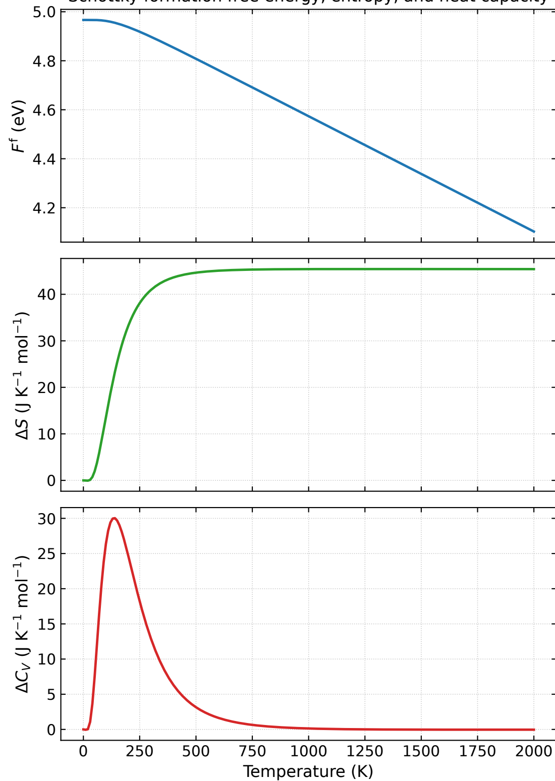
Schottky formation free energy, entropy, and heat capacity
