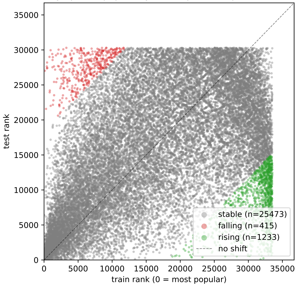
yelp2018 popularity shift (Spearman \rho = 0.512 )
