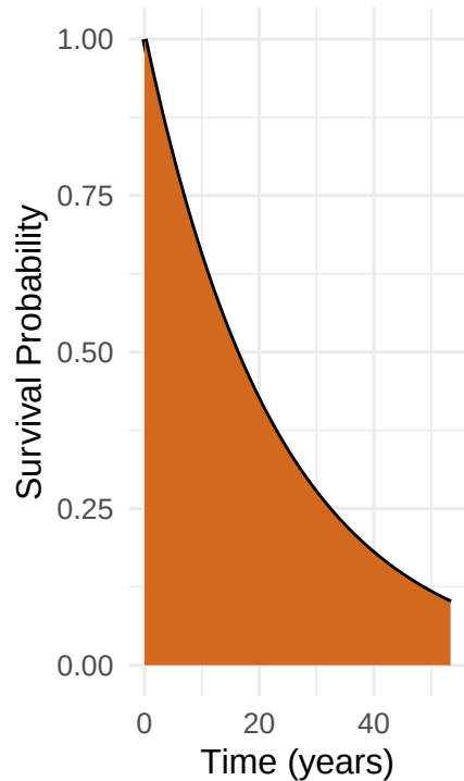
Survival Function
