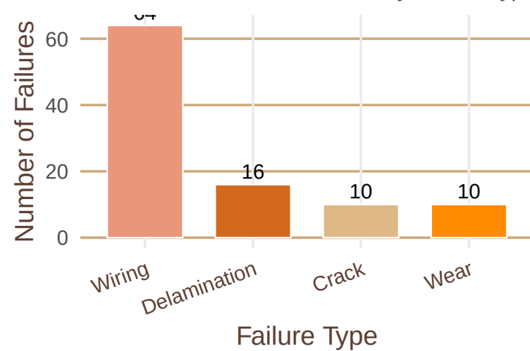
Number of Solar Panels Failed by Failure Type
