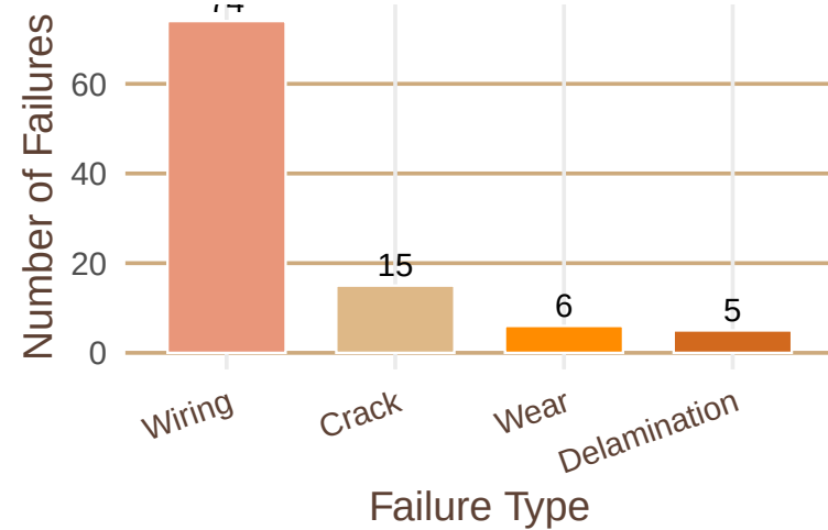
Number of Solar Panels Failed by Failure Type
