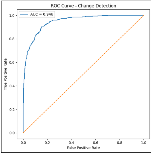
Fig 5: ROC Curve - Change Detection
