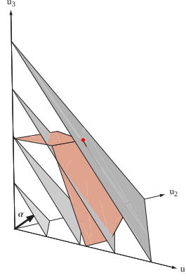
Figure 5.18: Surfaces of constant z = \mathbf{a}^t \mathbf{u} are shown in gray, while constraints of the form \mathbf{A}\mathbf{u} \leq \mathbf{b} are shown in red. The simplex algorithm finds an extremum of z given the constraints, i.e., where the gray plane intersects the red at a single point.
