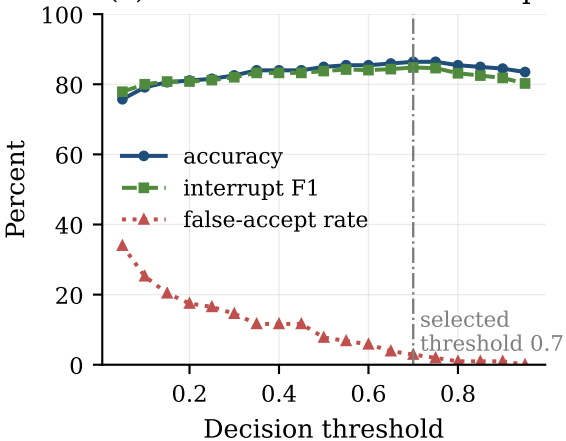
(a) Validation threshold sweep
