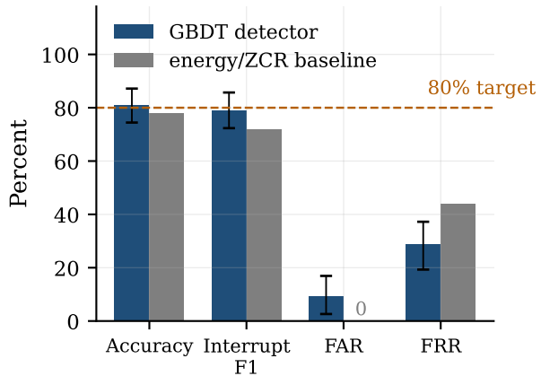
(b) Held-out test: 132 events, 22 sessions
