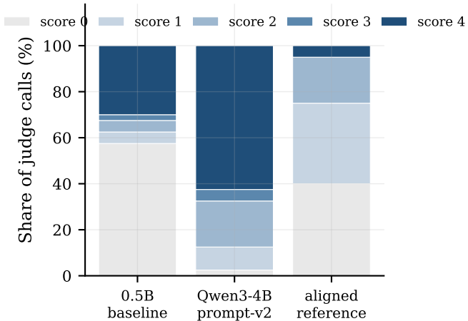
(b) Relevance score distribution (80 calls per arm)
