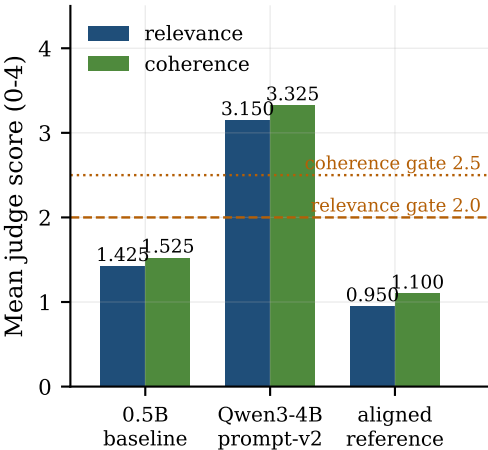
(a) Blinded arm means, n=40 rows
