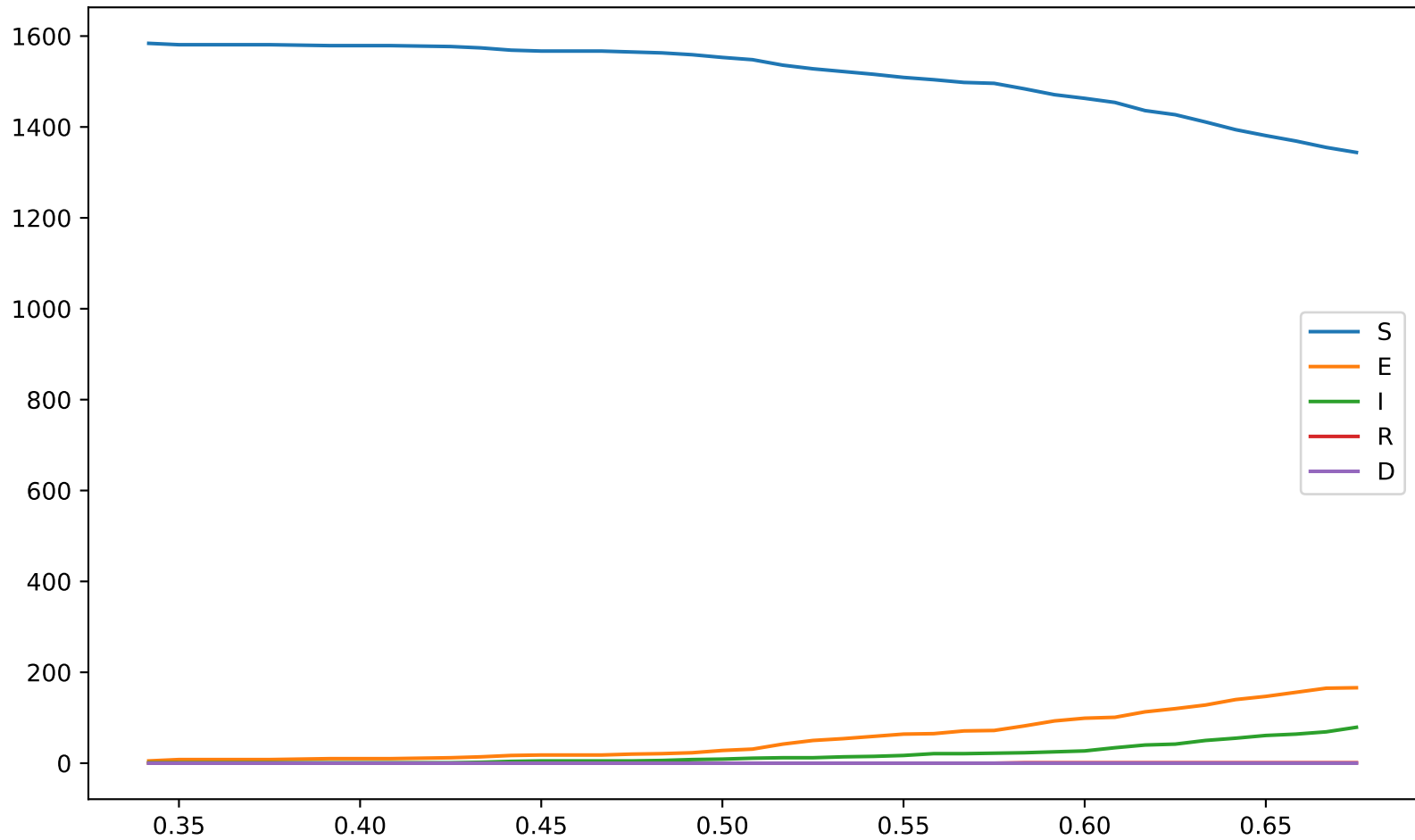
SEIRD Model
