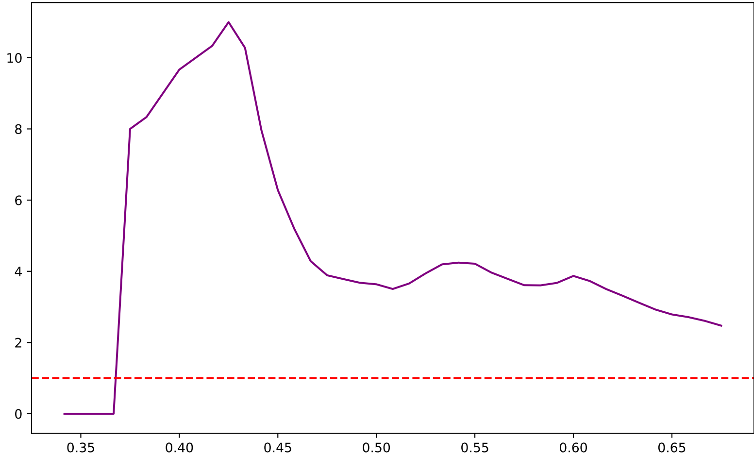
Reproduction Number
