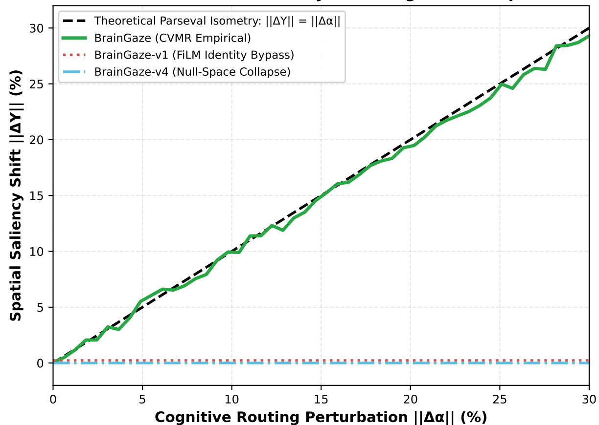
(c) Mathematical Isometry: Breaking the Null Space
