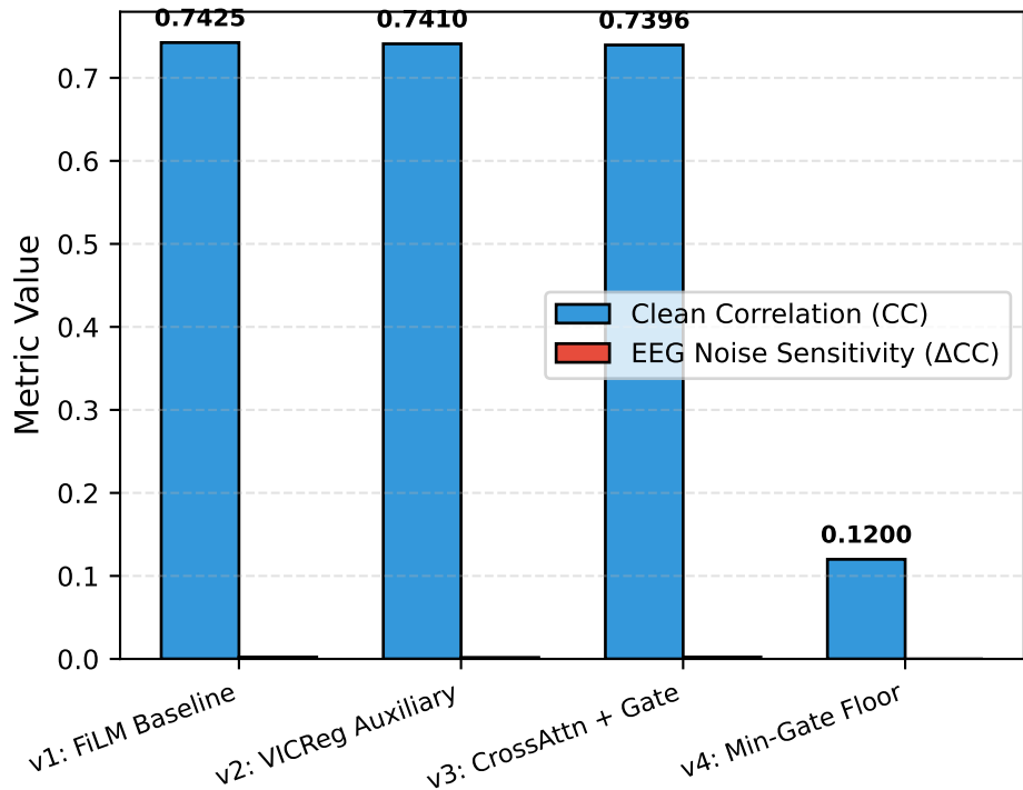
(a) BGD Architectural Iterations (CC vs. Noise Sensitivity)
