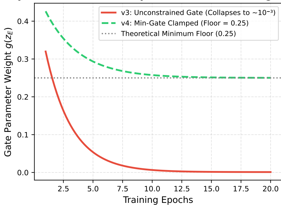
(b) Fusion Gate Dynamics Across Training
