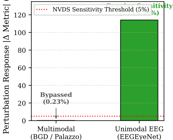
(b) Neural Pathway Sensitivity
