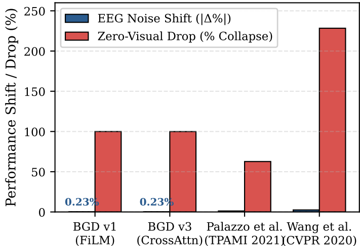
(a) Multimodal Paradigms: Modality Imbalance
