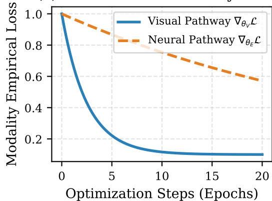
(b) Gradient Starvation Dynamics
