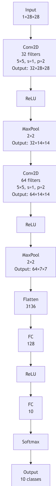
Figure 1: The CNN based architecture used for experiments
