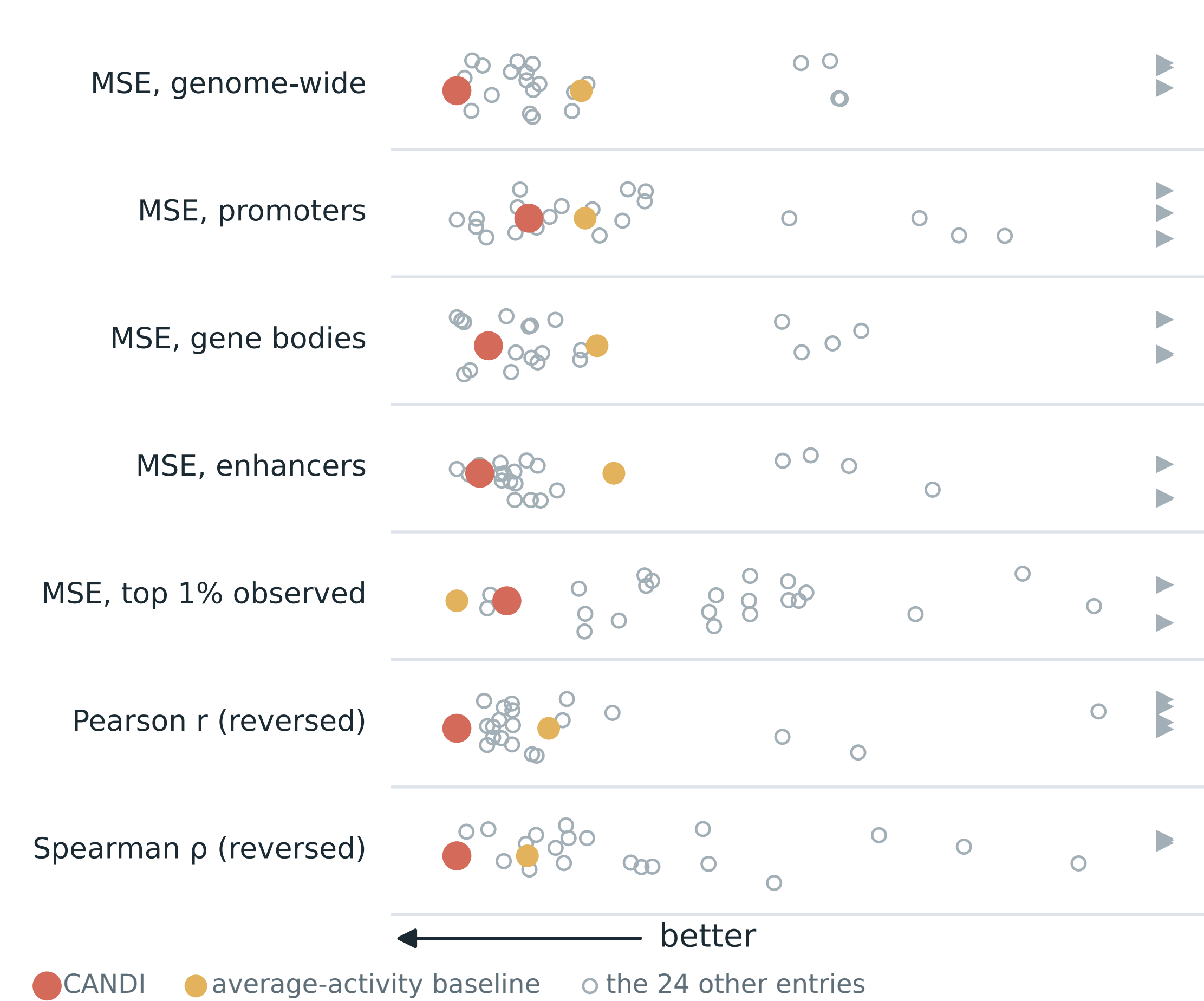
C Seven of the nine measures relative to the baseline, median over 51 experiments. CANDI is first on three and top 8 on the rest.
