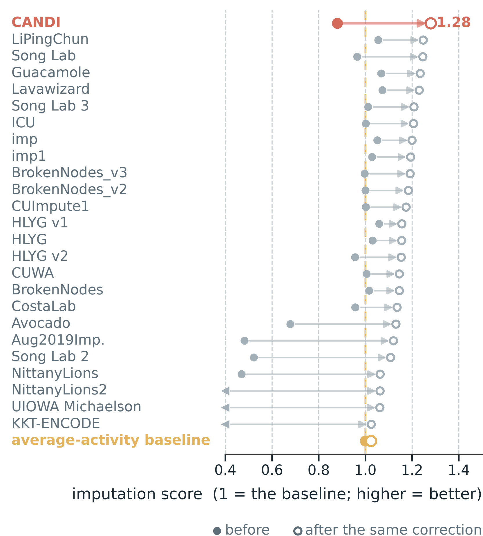
B Imputation score before (filled) and after (open) a correction that rescales each method's prediction and blends in the baseline. Every method improves; after it, CANDI is the best.
