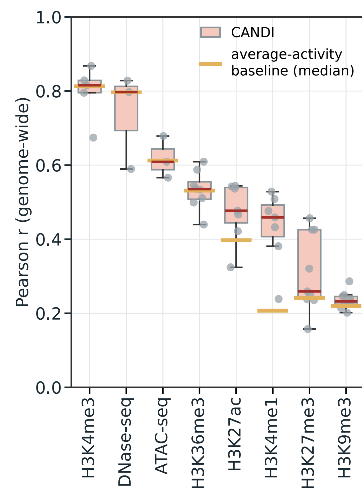
A CANDI's genome-wide Pearson r on the 51 blind-test experiments; mustard: the baseline's median.
