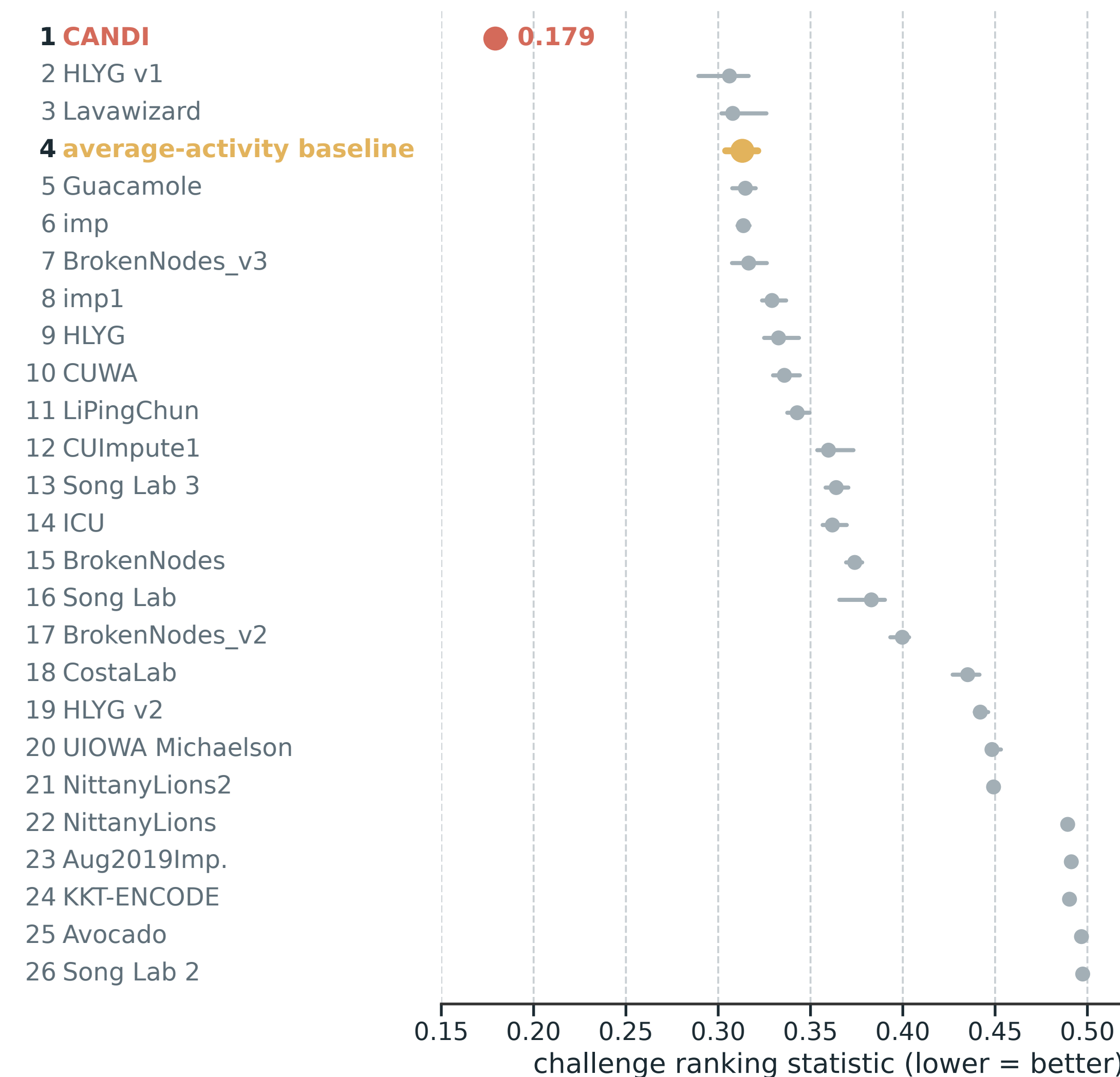
C The leaderboard with CANDI added: CANDI is first at 0.179 (bootstrap range 0.177–0.184), the next entry 0.306.
