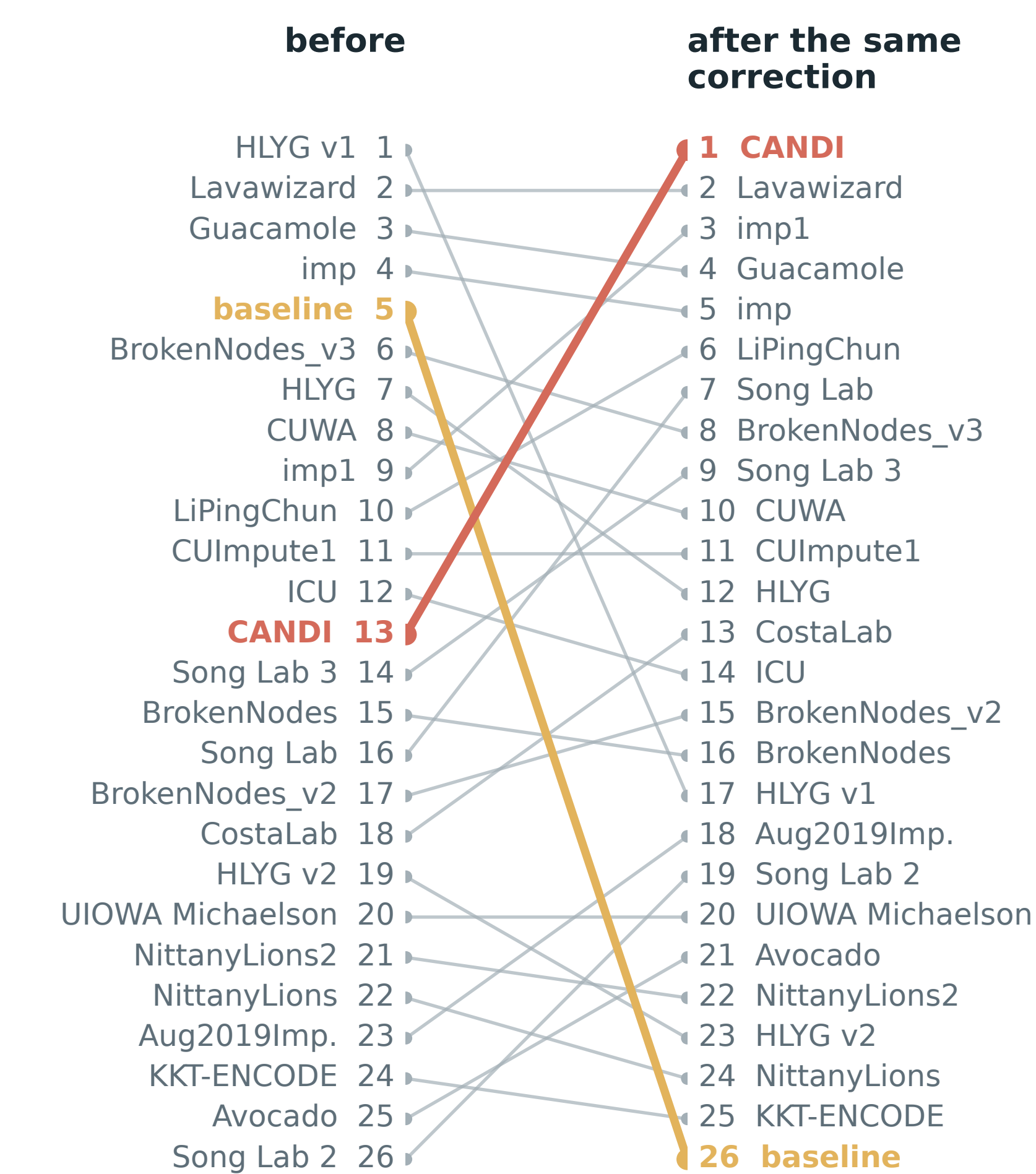
B Rank on the challenge's statistic before and after the same correction for every entry. CANDI rises from 13th to 1st; the baseline falls from 5th to last.
