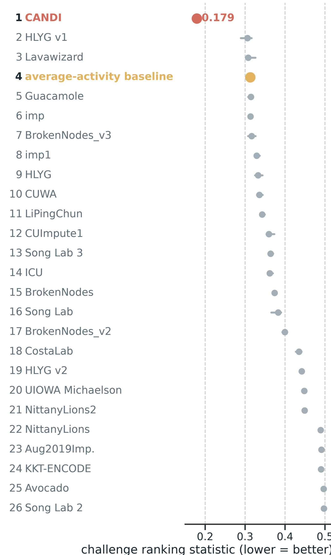
C The leaderboard with CANDI added: CANDI is first at 0.179 (bootstrap range 0.177–0.184), the next entry 0.306.
