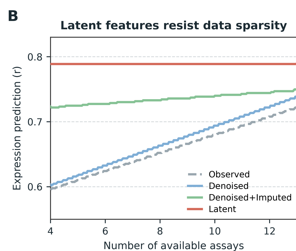
B Gene expression prediction as input assays are removed. Denoised+Imputed and Latent settings are robust to input sparsity.
