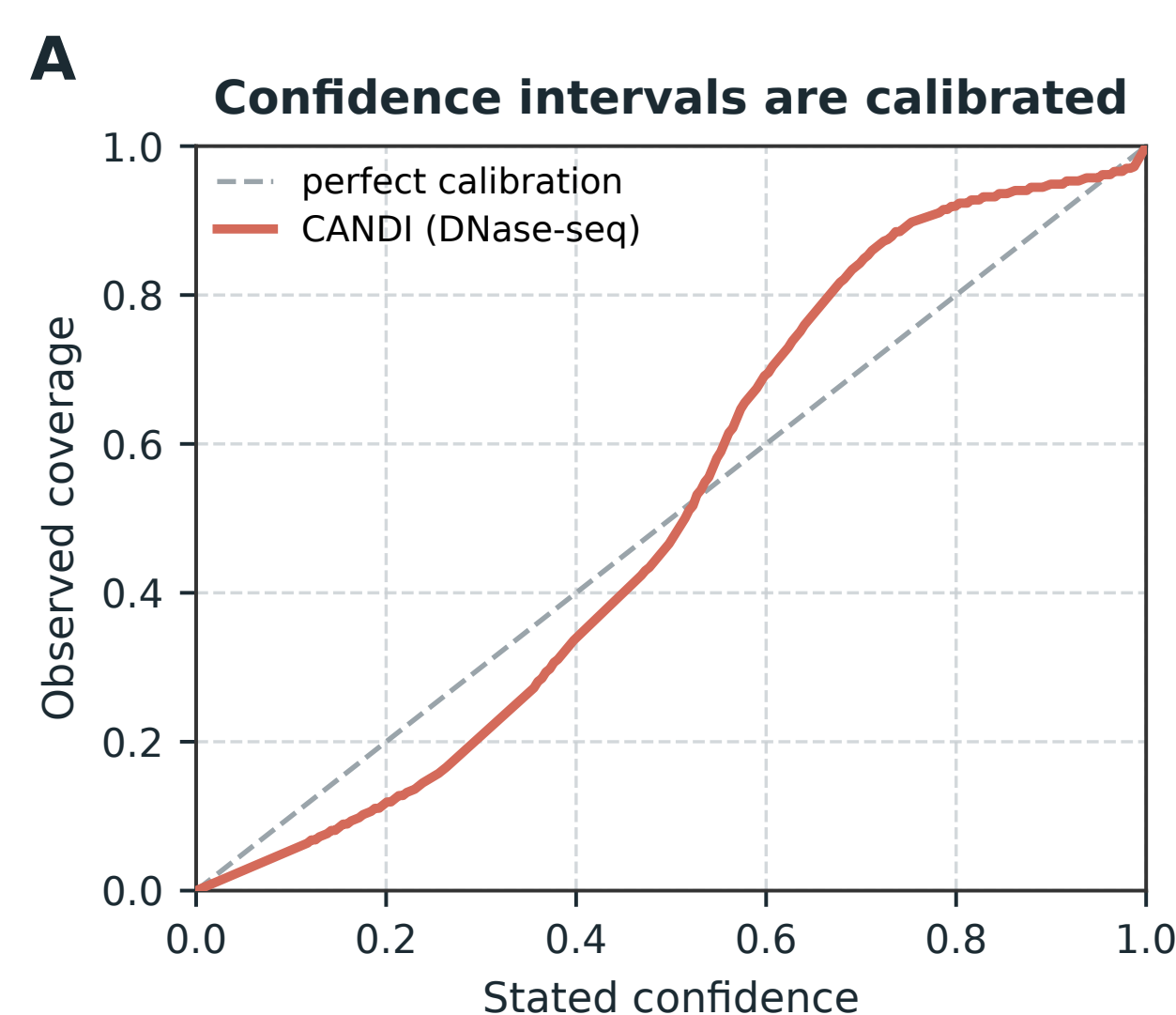
A Confidence calibration for DNase-seq (DND-41): predicted confidence level against the fraction of observed data within that interval.
