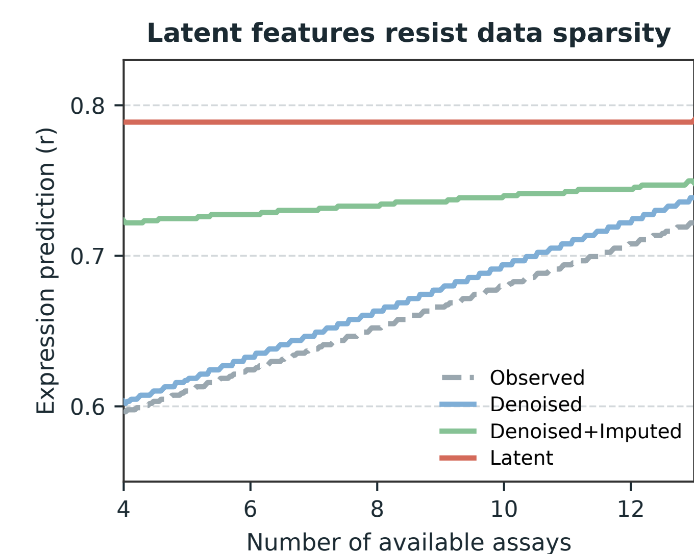
E Gene expression prediction as input assays are removed. Denoised+Imputed and Latent settings are robust to input sparsity.
