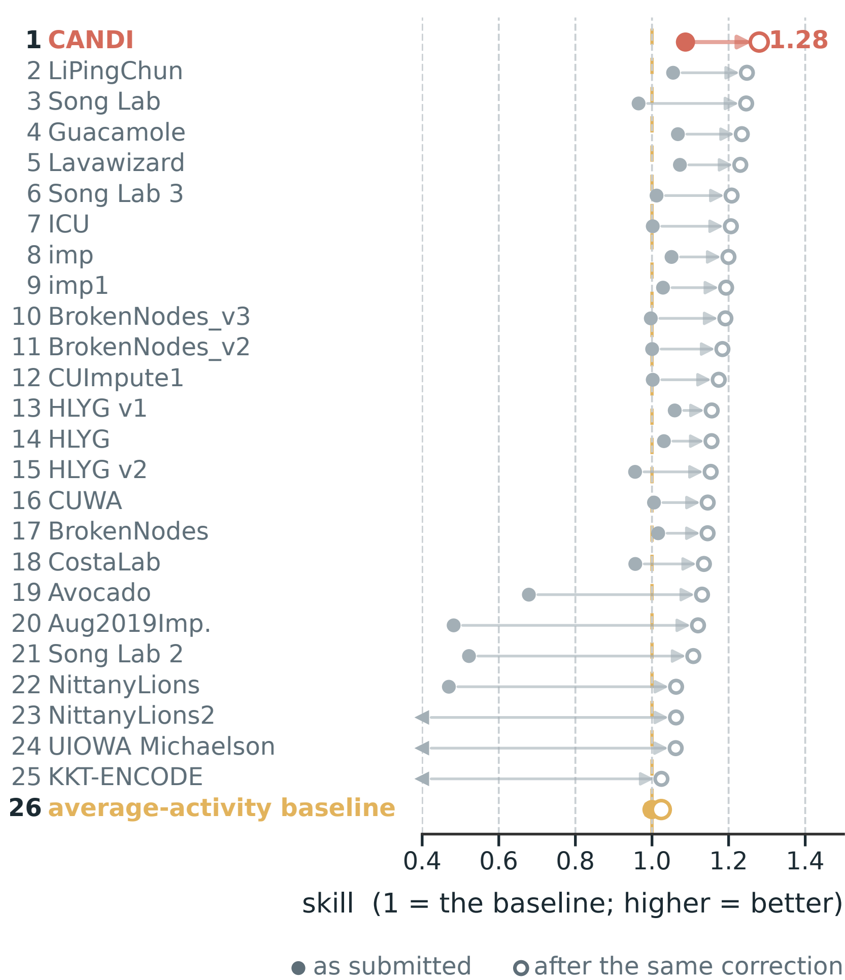
B Skill as submitted (filled) and after the same correction for every entry (open); 1 is the baseline. CANDI is first both ways.
