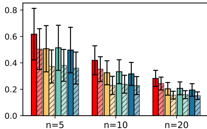
Balanced (B)
