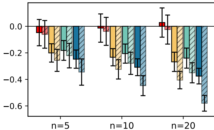
Moran (M)
