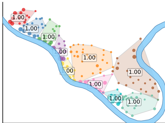
UP-balanced n-Means
