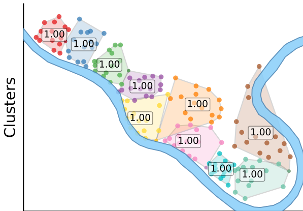
EP-balanced n-Means
