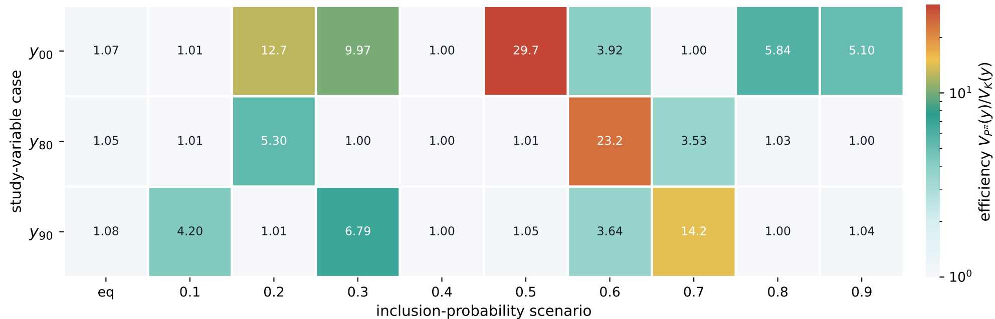
ABC efficiency for y under threshold stopping
