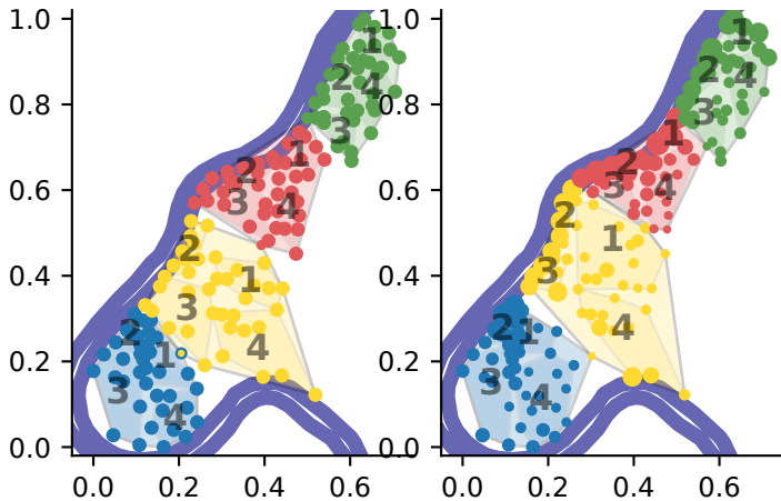
Meuse Population, Balanced Population, Balanced n-Means UP
