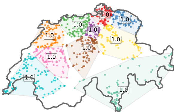
EP-balanced n-Means
