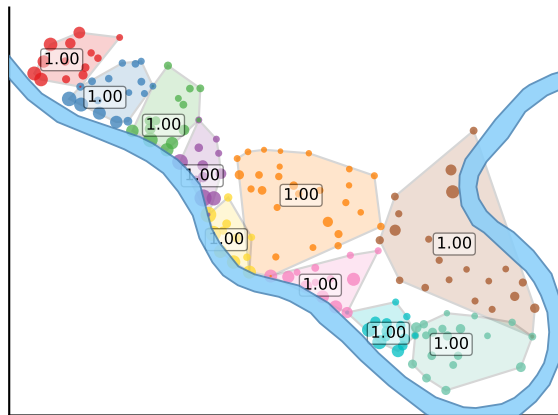
UP-balanced n-Means
