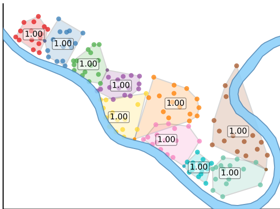
EP-balanced n-Means
